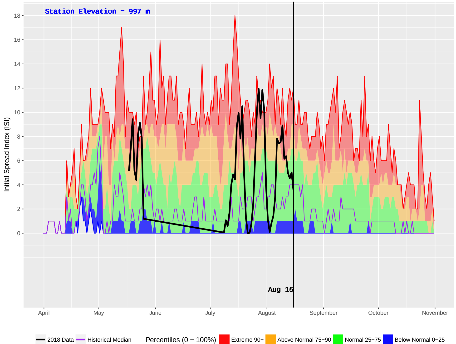
JERRY (190) : Historical (1988–2016) and Current (2018) Daily Initial Spread Index (ISI)
