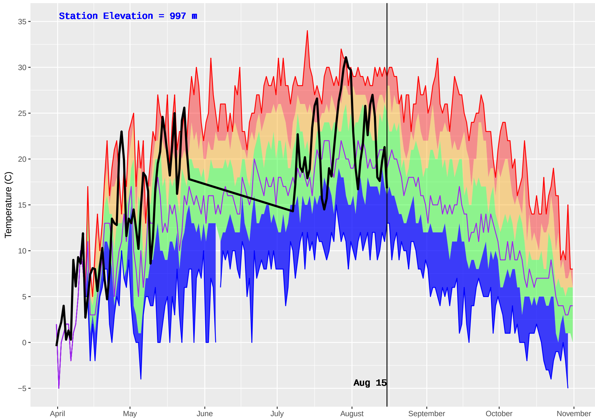
JERRY (190) : Historical (1988–2016) and Current (2018) Daily Temperature
