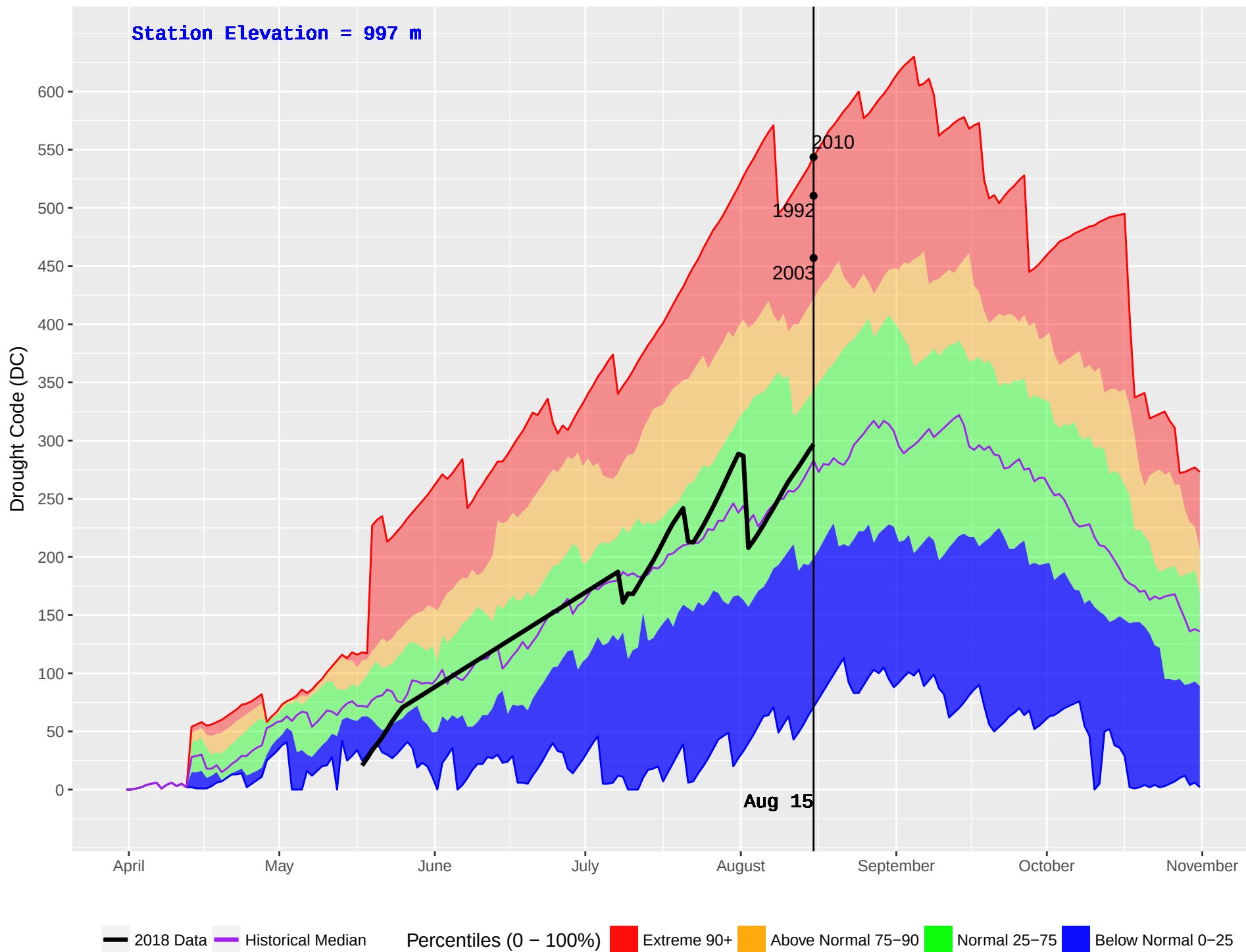
JERRY (190) : Historical (1988–2016) and Current (2018) Daily Drought Code (DC)
