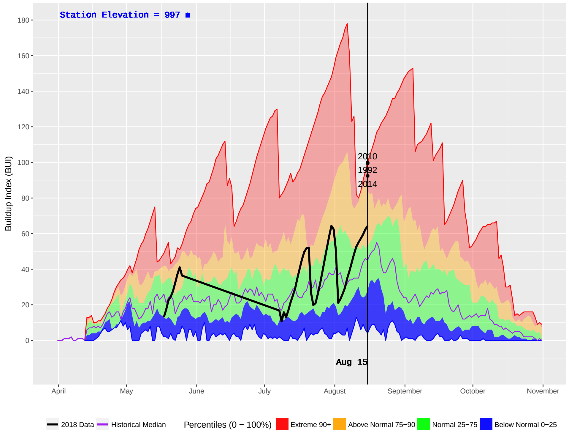
JERRY (190) : Historical (1988–2016) and Current (2018) Daily Buildup Index (BUI)
